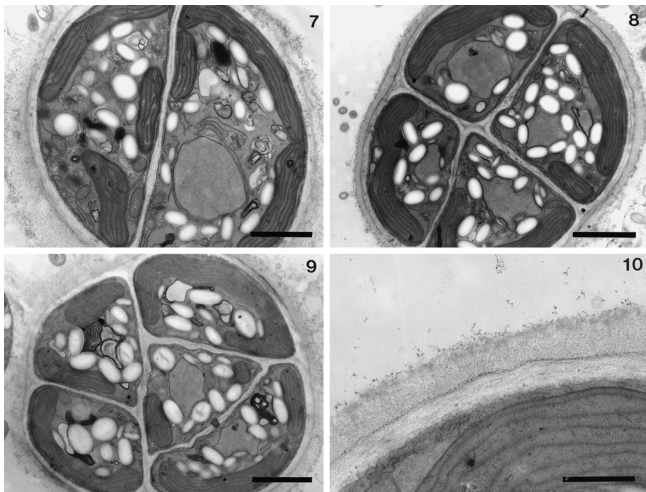
FIGS. 7–10. Ahnfeltiopsis furcellatus . Post-settlement development in laboratory culture. Scale bars = 3 \mu m (Figs. 7–9) and 500 \mu m (Fig. 10). FIG. 7. First mitosis in a 4-day-old sporeling. Immediate cell wall forms a pale septum dividing the two daughter cells and extends around the external face of each. This immediate cell wall is thin and surrounded by a thicker, fibrous external cell wall. Plastids have migrated toward the periphery and appear with clearly distinguishable thylakoids. Starch granules are less numerous, and the vacuole is still not apparent. FIGS. 8, 9. Second and third mitosis in a 4-day-old sporeling. Cell division is not accompanied by enlargement, and the resulting daughter cells are small. FIG. 10. Close-up of the two-layer outer cell wall of a 4-day-old sporeling. The fibrillar inner layer or immediate cell wall remains surrounded by a finely granular outer layer.
