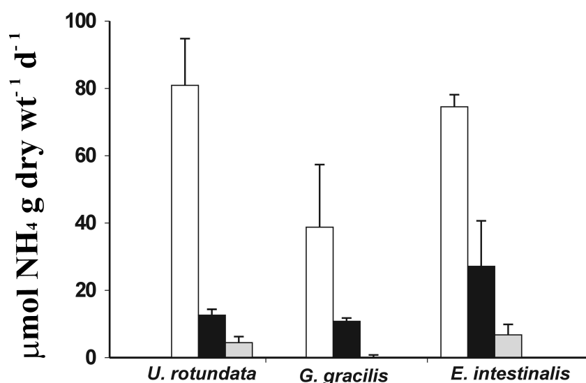
Figure 5. Integrated ammonium uptake rates of the species in the three-stage biofiltration design. White bars: first stage. Black bars: second stage. Grey bars: third stage. Data are means \pm SD (n = 2, 3).
