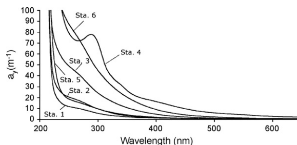
Fig. 7. UV/vis absorption spectra for CDOM at Stations 1–6 sampled on 8 September 2005.
