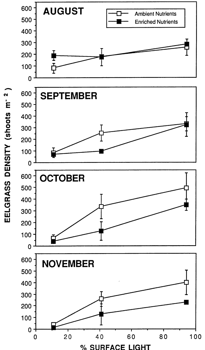
Fig. 5. Monthly eelgrass shoot density in mesocosm tanks during the shade-by-nutrient experiment, 1990. Values are the mean of two replicate tanks where shoot densities in three 0.02\text{-m}^2 quadrats per tank taken on each of three to five sampling dates per month ( \pm SE). Using ANOVA, we found date-by-light ( P < 0.05 ) and date-by-nutrient ( P < 0.01 ) interactions to be significant, indicating that both light and nutrient effects became significant over time.
