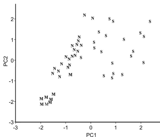
Figure 4 Principal component analyses of physical data collected at each site in the Black Point area of Biscayne Bay.
