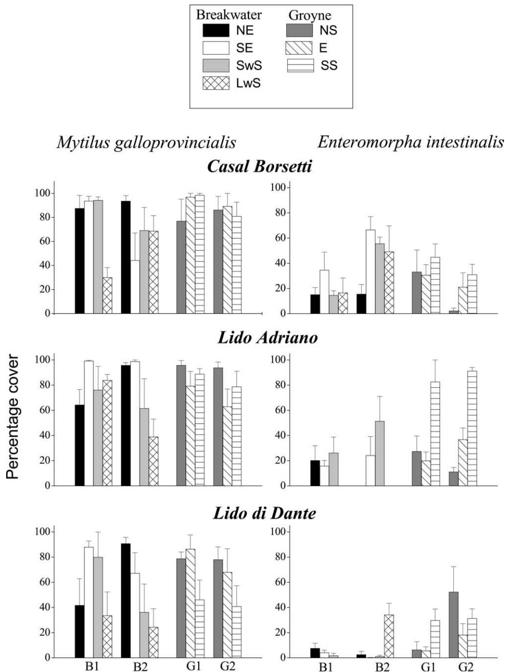
Fig. 2. Percentage cover (+SE, n = 5 ) of Mytilus galloprovincialis and Enteromorpha intestinalis at three stations and at different positions around groynes and breakwaters. At each station, sampling was done at all positions around two breakwaters (B1, B2) and two groynes (G1, G2). Symbols for positions are coded as in Fig. 1C.
