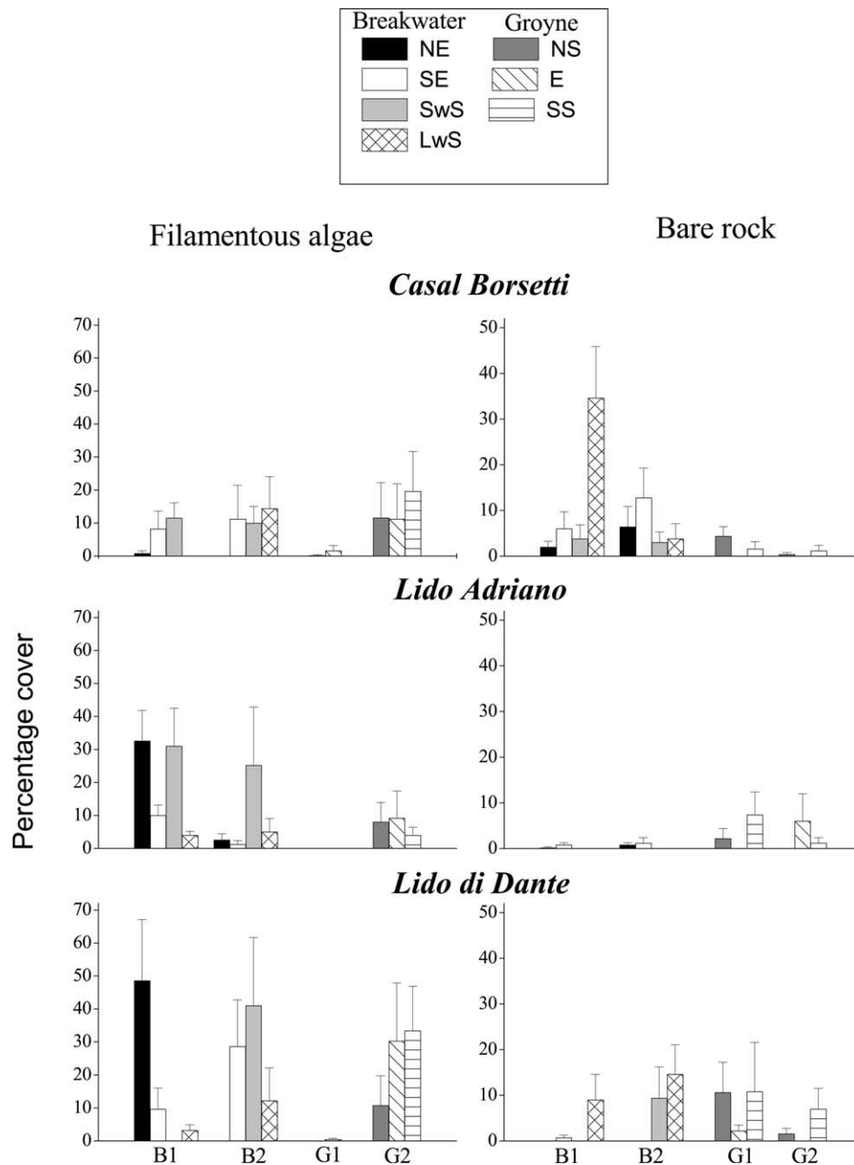
Fig. 3. Percentage cover (+SE, n = 5 ) of filamentous algae and bare rock at three stations sites and at different positions around groynes and breakwaters. At each station, sampling was done at all positions around two breakwaters (B1, B2) and two groynes (G1, G2). Symbols for positions are coded as in Fig. 1C.
