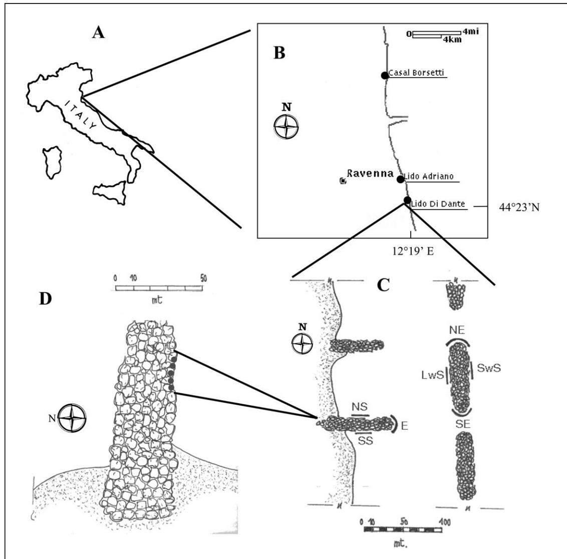
Fig. 1. (A) Location of the study area, (B) location of the three study stations (Casal Borsetti, Lido Adriano and Lido di Dante), (C) location of areas at different positions around groynes (NS, north side; E, end; SS, south side) and breakwaters (NE, north end; SE, south end; SwS, seaward side; LwS, landward side) and (D) example of location of replicate plots in one area (10 m long transect). In (C) and (D), symbols for areas and plots are not to scale.
