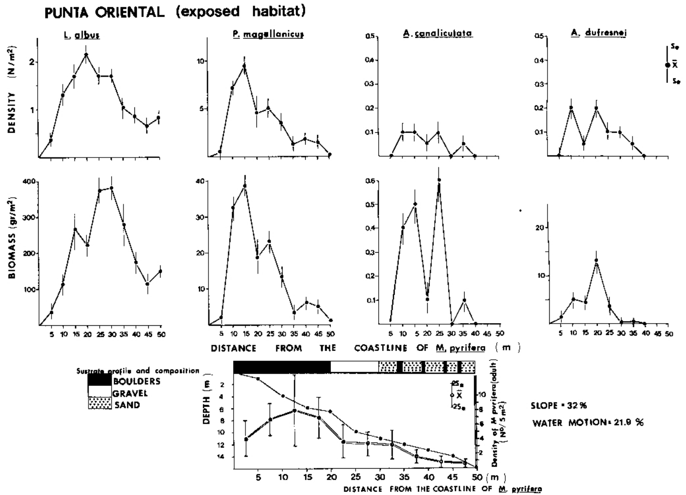
Fig. 3. Density and biomass distribution of the 4 species of sea urchins at the exposed habitat in the forest of Macrocytis pyrifera in Puerto Toro, southern Chile. Units in ordinate different for the various species. Substratum profile (solid circles) and composition and density of adult plants of M. pyrifera (open circles) on sampling transect given in lower diagram
