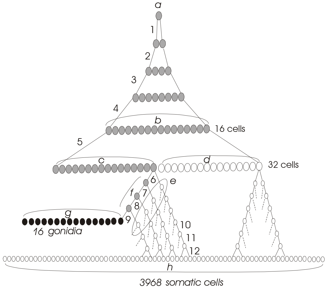
Figure 4. Schematic representation of the development and germ/soma separation in an asexual V. carteri . Gray ellipses denote the totipotent and multipotent cell lineages: the asexual spore, i.e., gonidia (“a”), the 16 totipotent blastomeres (“b”), the germ-line precursors (“c”), and the germ-line blastomeres (“f”); white ellipses indicate unipotent (i.e., the somatic blastomeres and initials, “d” and “e”) and terminally differentiated somatic cells (“h”), and black ellipses indicate terminally differentiated reproductive cells, i.e., gonidia (“g”). Note somatic cells (“h”) have two distinct origins, from germ-line blastomeres (“f”) via asymmetric divisions and from somatic blastomeres (“b”) via symmetric divisions. Numbers mark the succession of cell divisions in the embryo. Cells are not represented at scale (“a” is ca. 2^9 -fold larger than “g”, and there is a \frac{1}{2} -reduction in cell size with every symmetric cell division); all divisions take place under the mother cell wall, in a rather rapid fashion without intervening growth (i.e., palintomy and multiple fission).
