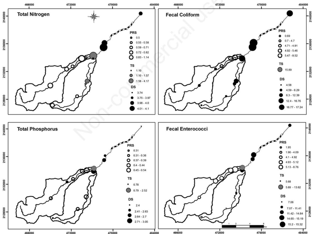
Fig. 2. Total nitrogen, total phosphorus, fecal coliform bacteria and fecal enterococci ( n=16 , mean values). The color of the circles indicate differences between sites according to the Mann-Whitney Test ( \alpha=0.05 ): white circles indicate potential reference sites PRS); grey circles indicate transition sites (TS); black circles indicate degradation sites (DS) in the Magdalena and Eslava Rivers. Site abbreviations correspond to those shown in Fig. 1.
